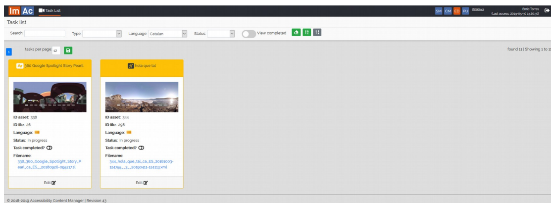
Figure 1: Editor interface
